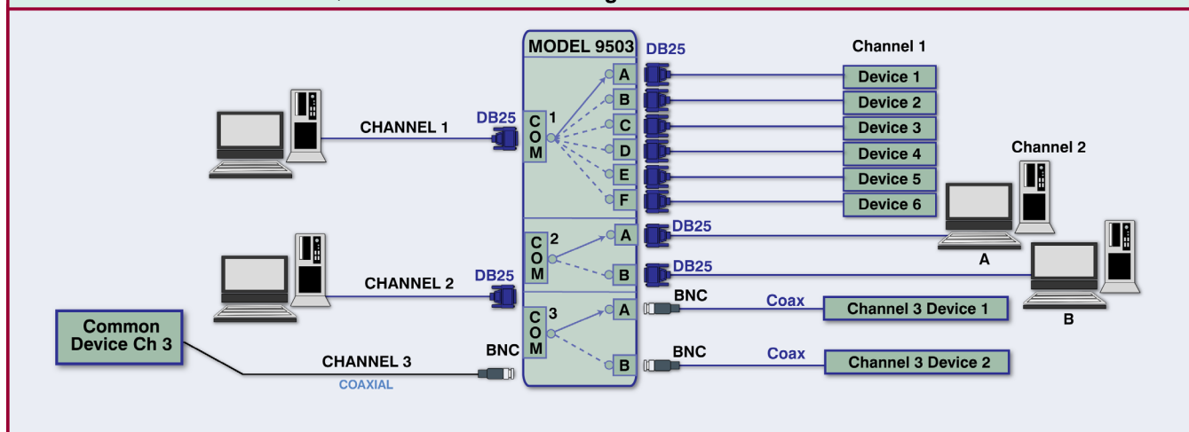
Model 9503 Tri-Channel DB25/BNC Switch Function Diagram
