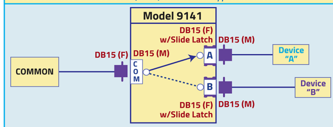
LineSelect® Model 9141 DB15 A/B (F/F/M) Switch Module Application w/Slide Latch
