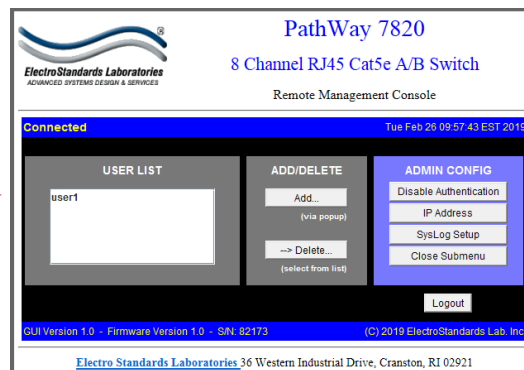
Figure 4: The Admin-only section is in Admin Submenu.
