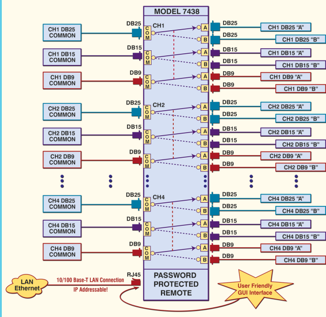
PathWay® Model 7438 4-Channel DB25/DB15/DB9 A/B Switch Application: w/ Telnet & GUI
