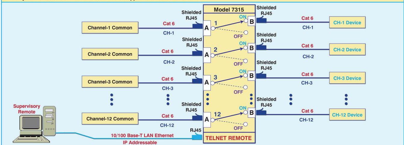
PathWay® Model 7315 Cat6 Shielded RJ45 On/Off Application with Telnet Remote
