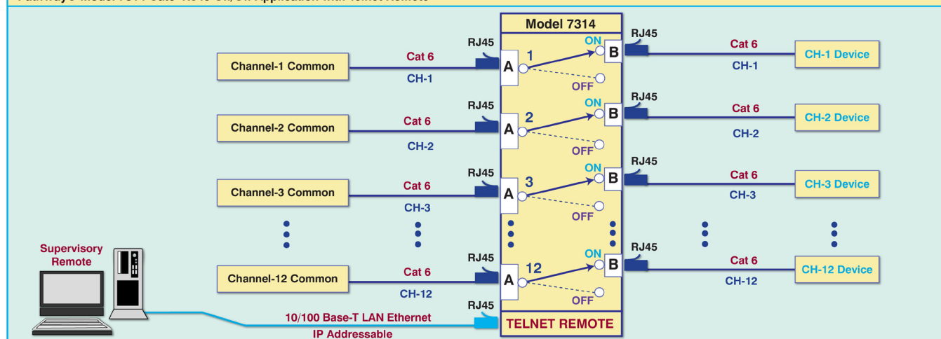
PathWay® Model 7314 Cat6 RJ45 On/Off Application with Telnet Remote
