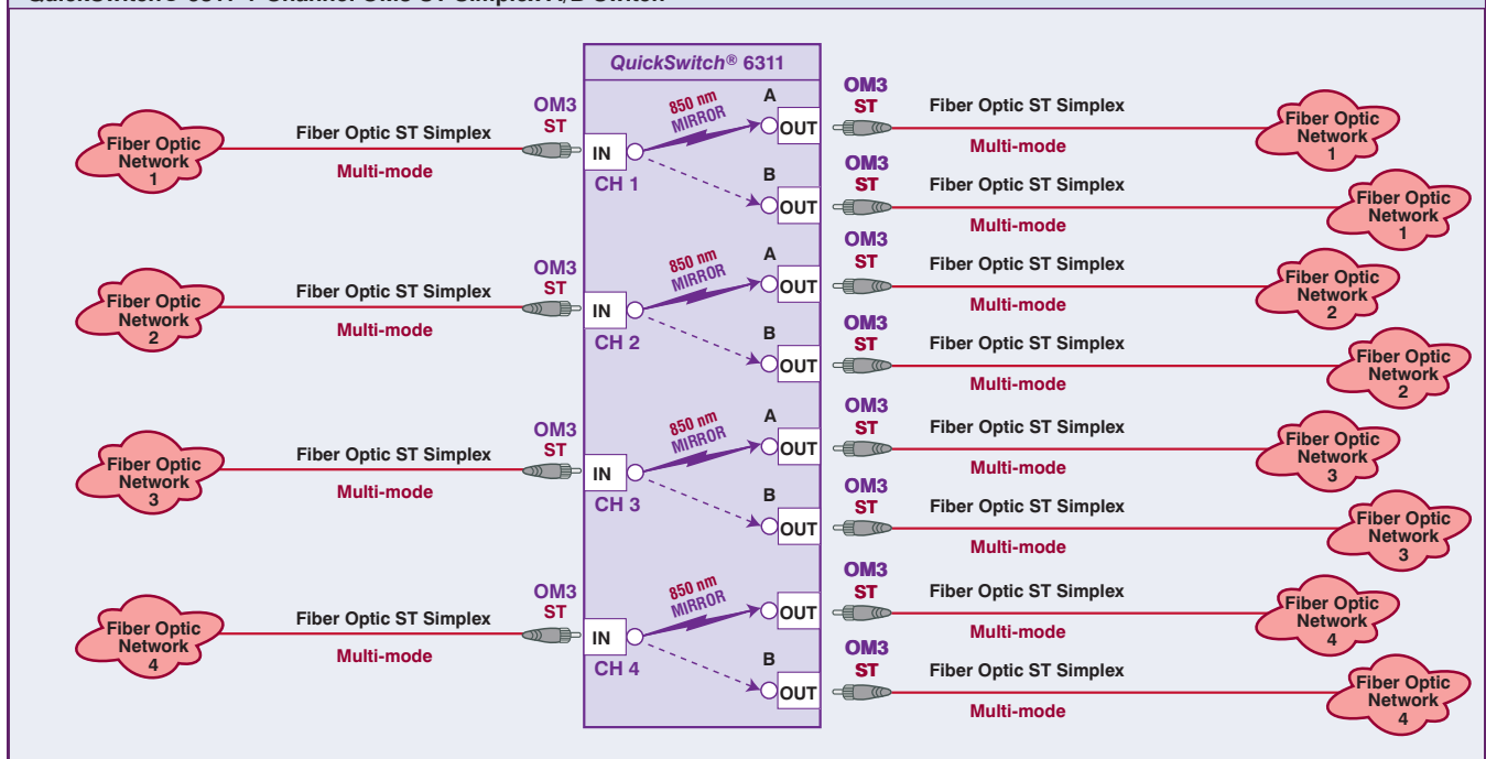
QuickSwitch® 6311 4-Channel OM3 ST Simplex A/B Switch
