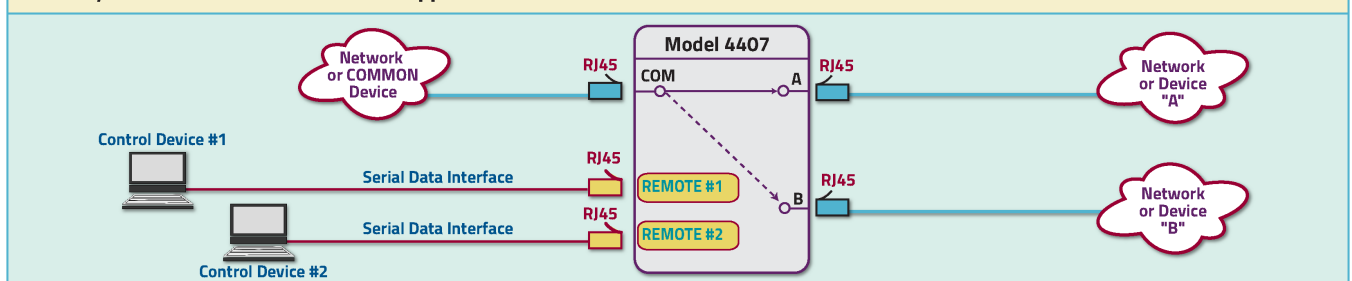
PathWay® Model 4407 RJ45 A/B Switch Application w/Dual Remotes
