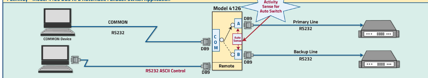
PathWay® Model 4126 DB9 A/B Automatic Fallback Switch Application
